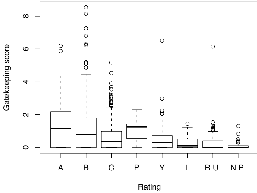
Figure 2: Boxplot of gatekeeping score by NRF-rating. The boxes comprise the lower and upper quartile of respective distributions, the median is marked with a bar, hinges extend the boxes by at most 1.5 the interquartile range. Three researchers, i.e. two A and one B researchers with gatekeeping score larger 10, are not displayed.
