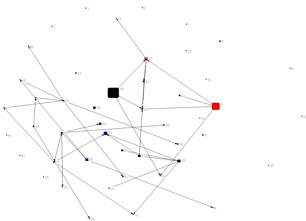
Appendix 2A. Academic network of strong tie based on Centrality (betweenness) and academic performance
