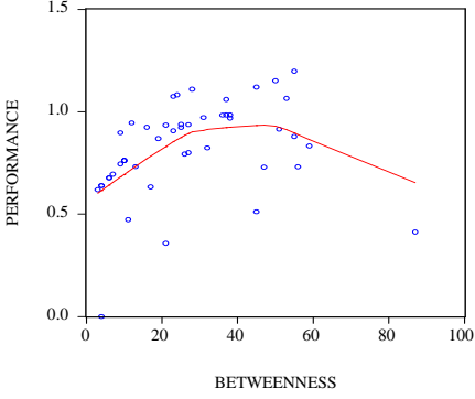
Graph 2A- Effect of centrality (betweenness) in academic network on academic performance
