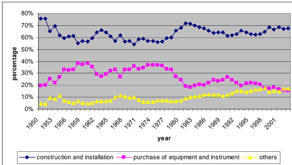
Figure 3: Total Investment in Basic Construction, by Content Category, 1950-2003
